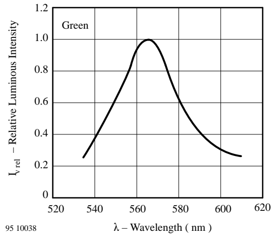
Figure 21. Relative Luminous Intensity vs. Wavelength
